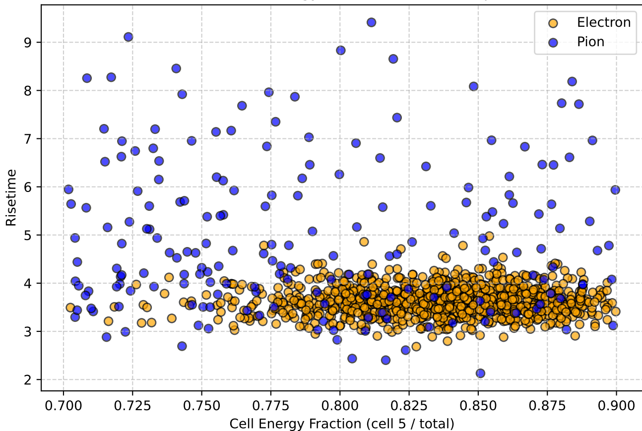
Risetime vs Cell Energy Fraction for 2.0GeV particles
